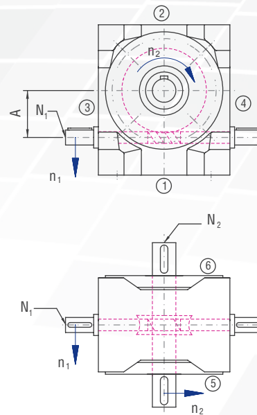
Figure 9.3.3-2; Shaft designations
